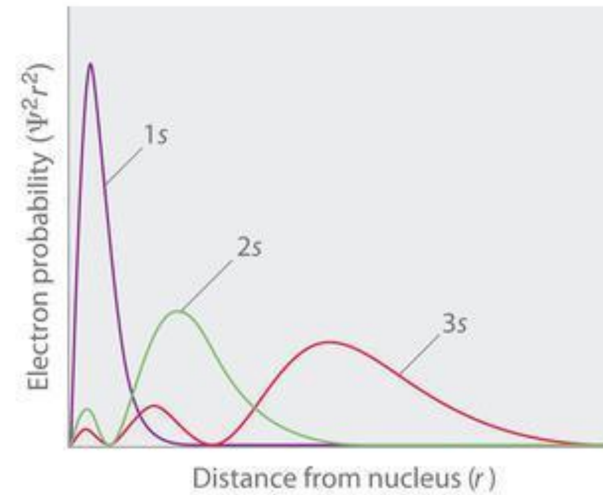
(c) Radial probability
